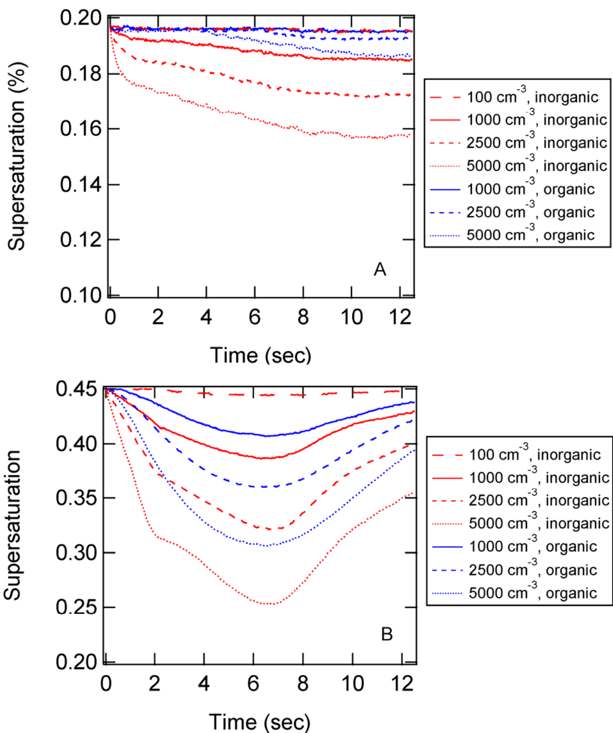
Figure 11ab. Modeled supersaturation time series during the chamber growth cycle for varying aerosol number concentration and two particle types (inorganic: Van't Hoff factor = 3, Density = 1777 kg m -3 , Molecular Weight = 117 g mol -1 ; organic: Van't Hoff factor = 1, Density = 1200 kg m -3 , Molecular Weight = 250 g mol -1 ) One lognormal size mode with D = 147 nm and \sigma = 1.34 was assumed. Panels A and B were initialized with a supersaturation of 0.197% and 0.450%, respectively.
