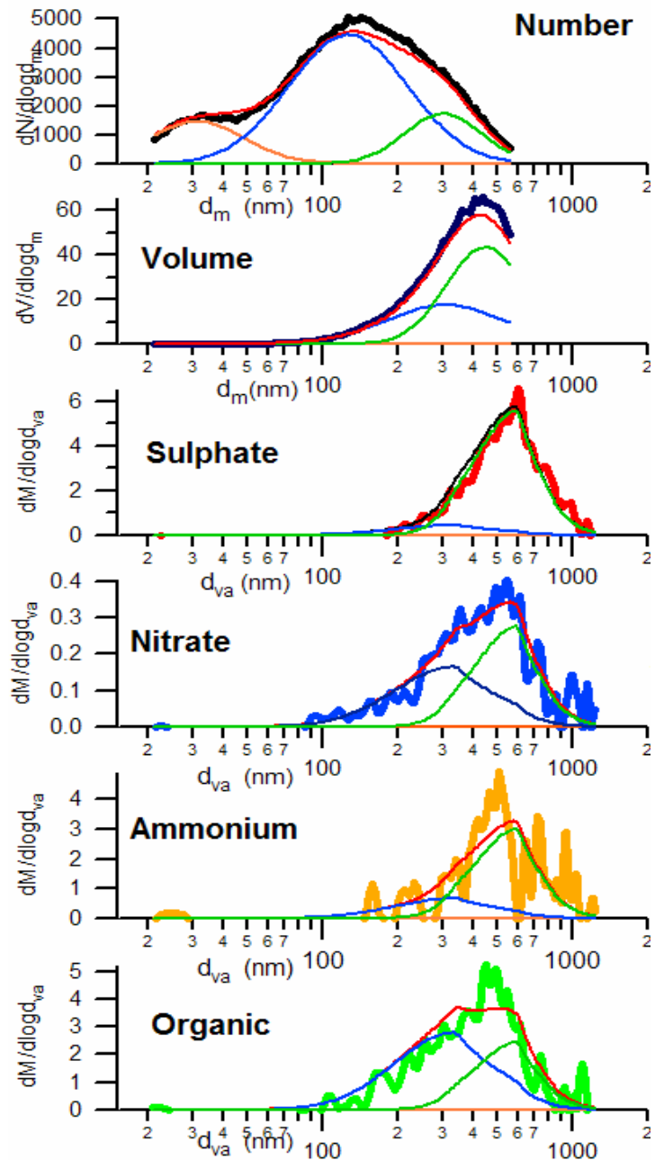
Figure 8. Observed aerosol size distribution (number, volume and component mass) and lognormal fits for the time period from 0930 EST July 16 2003 to 1130 EST July 16 2003.
