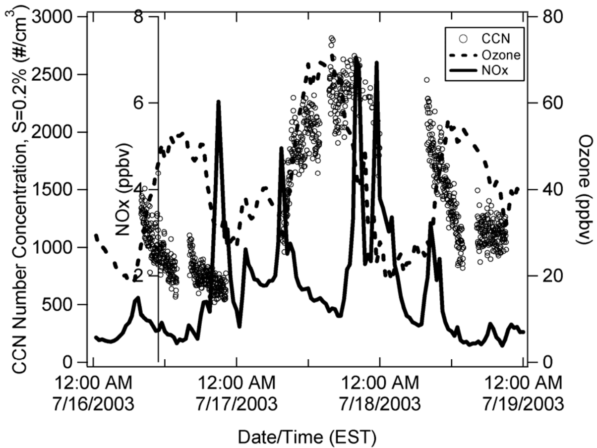
Figure 6. Observed time series for O 3 , NO x and CCN number concentration (S = 0.2%).
