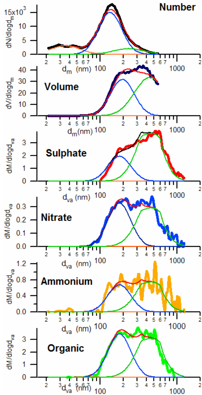
Figure 9. Observed aerosol size distribution (number, volume and component mass) with lognormal fits for the time period from 1030 EST July 17 2003 to 1330 EST July 17 2003.
