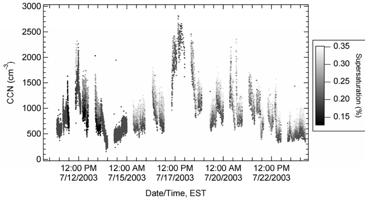
Figure 1. Observed CCN number concentration time series color-coded as a function of percentage supersaturation.
