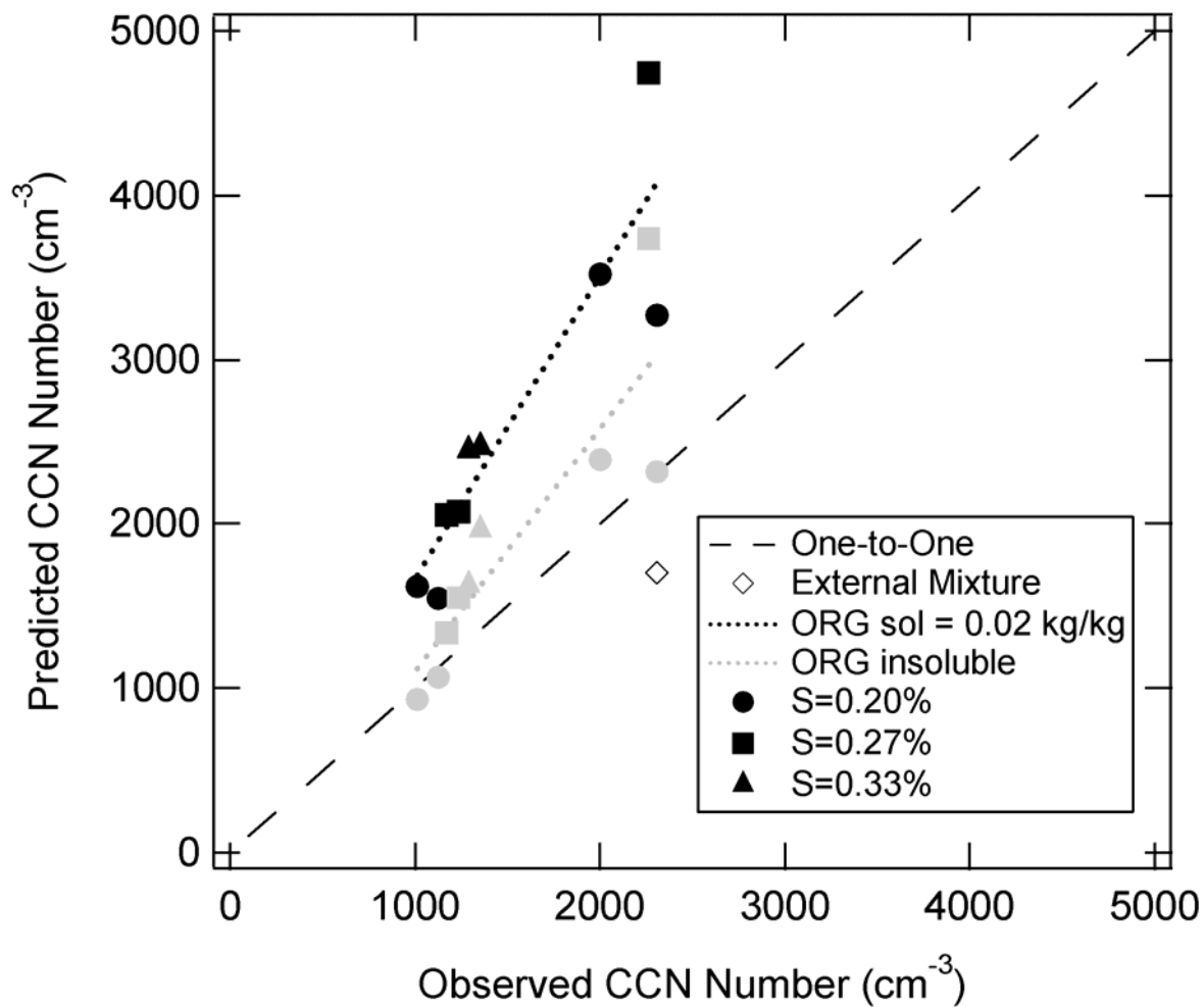
Figure 10. Comparison between CCN predicted and CCN observed for selected case studies. The symbol type represents chamber supersaturation (circle, 0.20 %; square, 0.27 %; triangle, 0.33 %). The symbol contrast represents sensitivity simulation parameters (dark points for ORG solubility=0.02 kg kg -1 ; light points for ORG solubility=1x10 -5 kg kg -1 ). Dashed lines are least-squares linear best fits through like contrast points. The open diamond point is the result of a simulation assuming external mixing for mode 2 of case 3.
