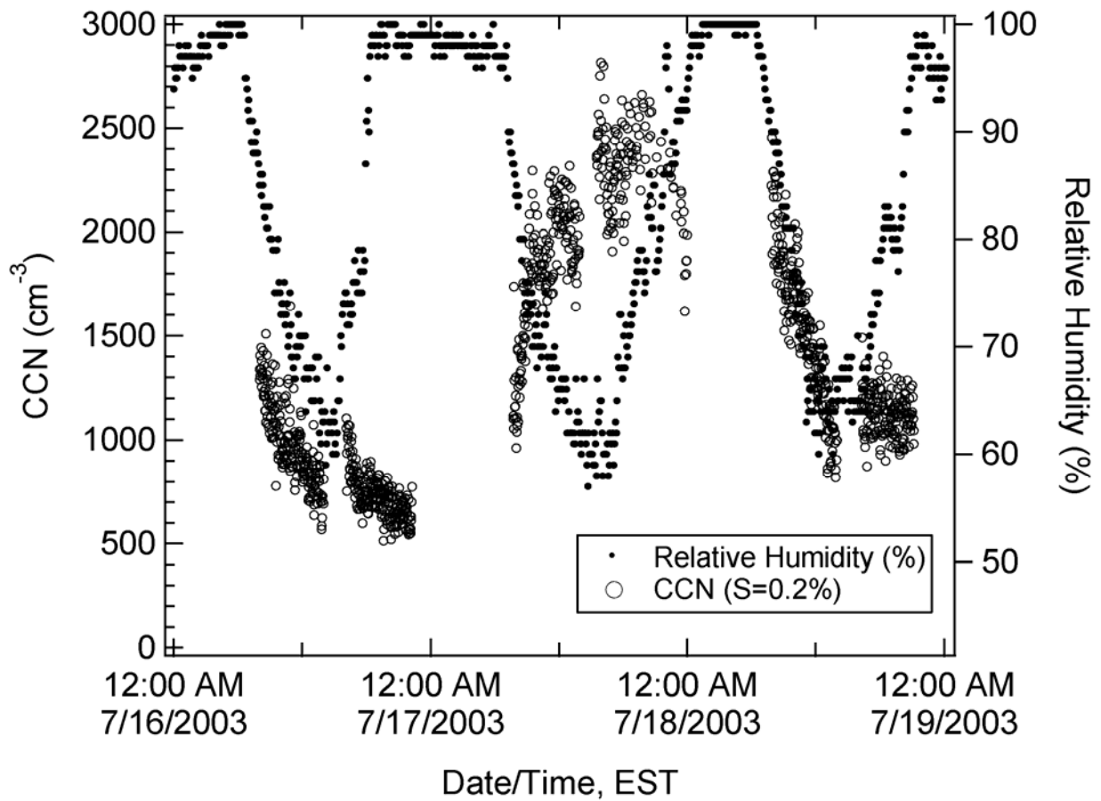
Figure 7. Observed time series for relative humidity and CCN number concentration ( S = 0.2\% ).
