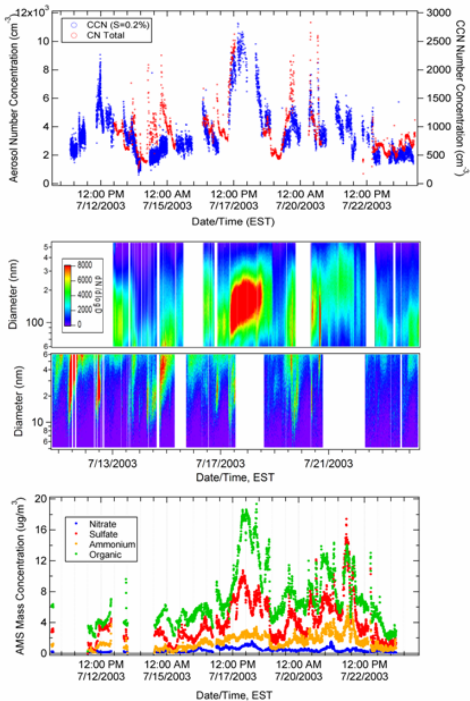
Figure 4abc. Observed time series for total aerosol number concentration and CCN number concentration ( S = 0.2\% ) (panel A), aerosol size distribution (panel B), and aerosol component mass concentrations (panel C).
