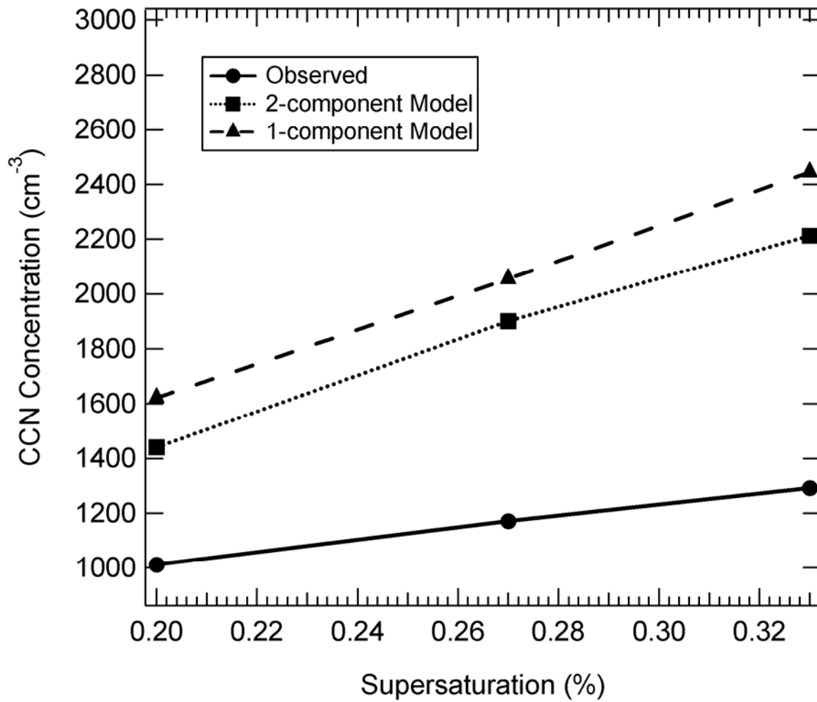
Figure 12. Observed and predicted CCN supersaturation spectra for case 1 with the 1 ORG component and 2 ORG component versions (ORG1 25 % by mass, sol=0.3 kg/kg; ORG2 75 % by mass, sol=0.005 kg/kg) of the chamber model.
