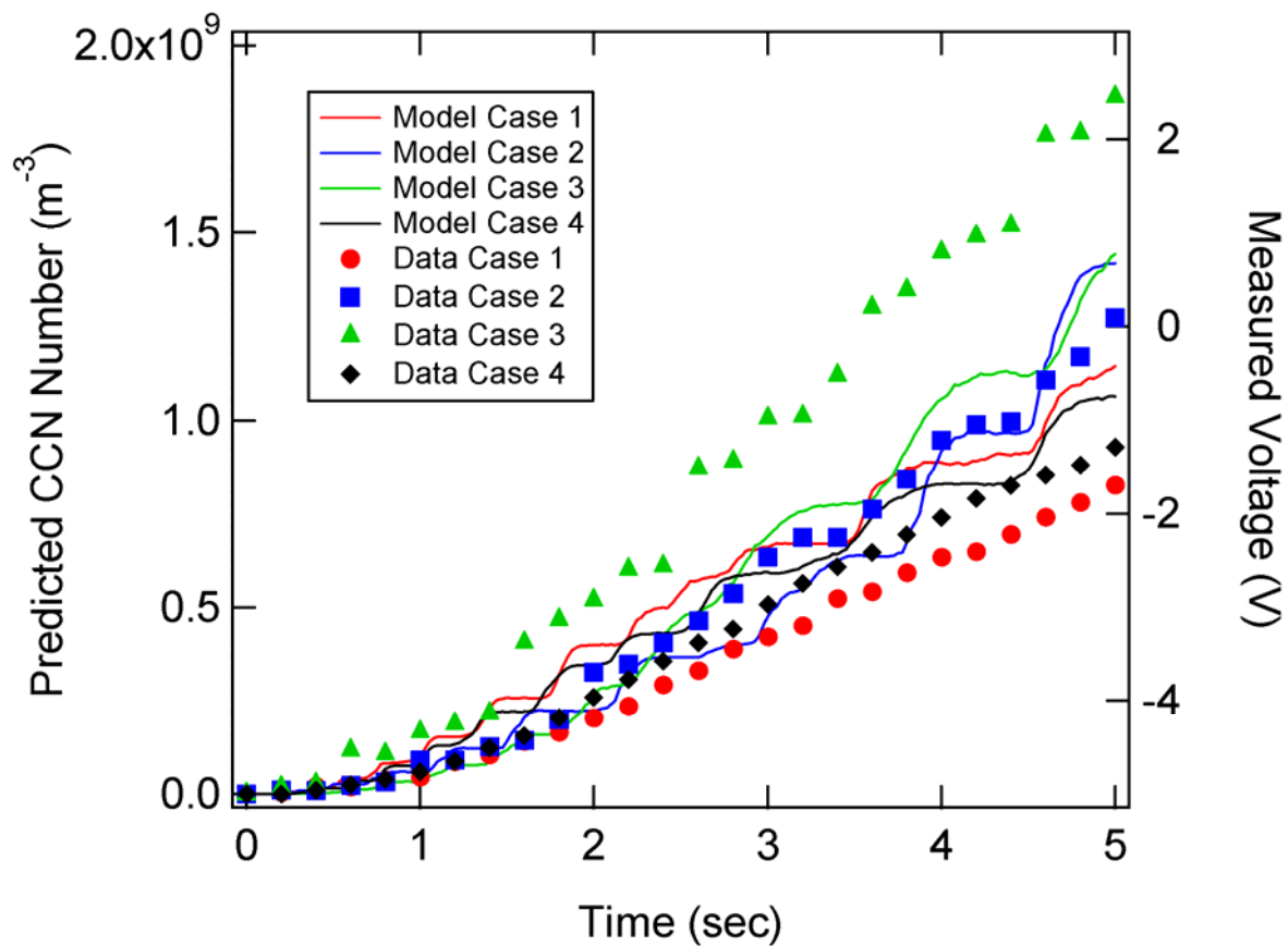
Figure 2. Measured scattering voltage recorded by the CCN counter during the first 5 sec of activation period averaged for each of the 4 case studies. An offset voltage was added to each trace so that all four cases started at -5 V. Also included are model-derived CCN number concentrations along the centerline of the CCN chamber.
